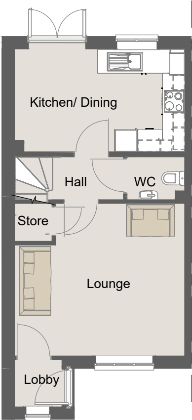
Ground Floor 1 : 100
