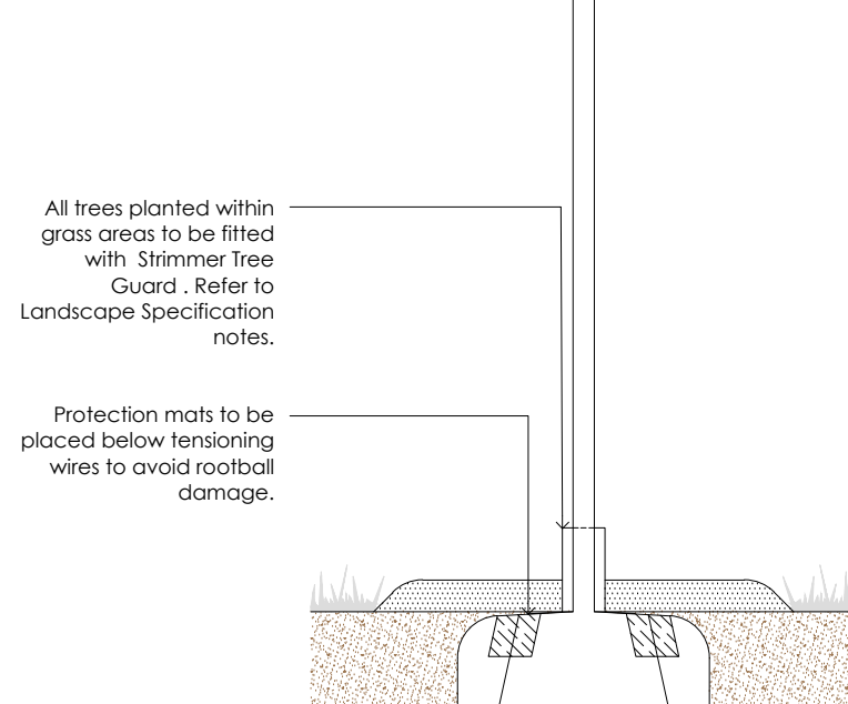
Detail 5 - Typical Semi Mature 25cm+ Girth Support Detail
