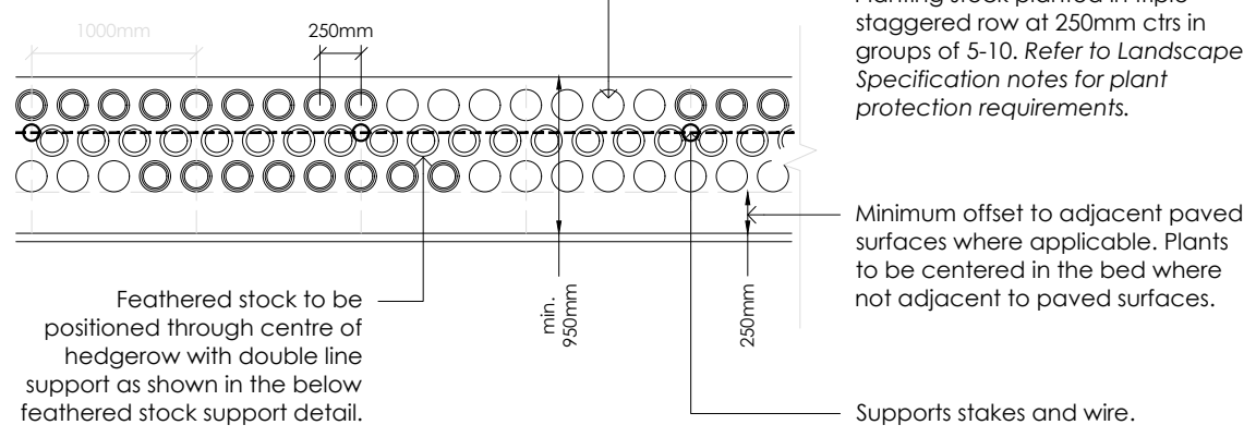
Detail 9 - Typical Native Hedgerow Triple Staggered Layout (N.T.S.)
