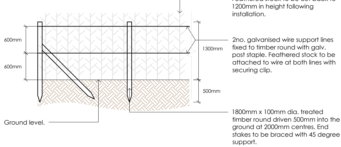
Detail 10 - Typical Feathered Stock Support Detail (N.T.S.)
