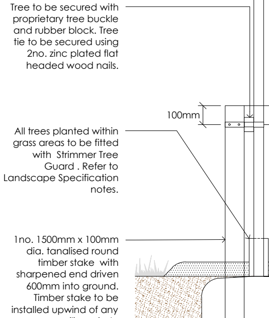
Detail 4 - Heavy Standard to Semi Mature Support Detail
