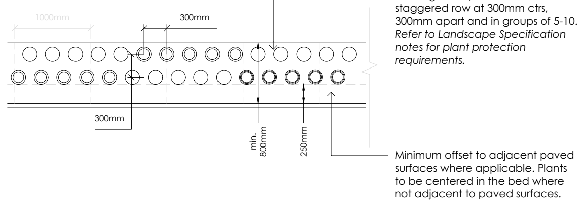
Detail 8 - Typical Native Hedgerow Double Staggered Layout (N.T.S.)
