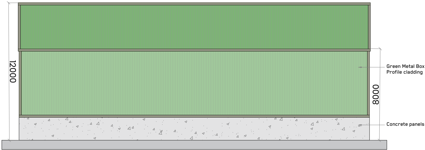
1:200 East Elevation
