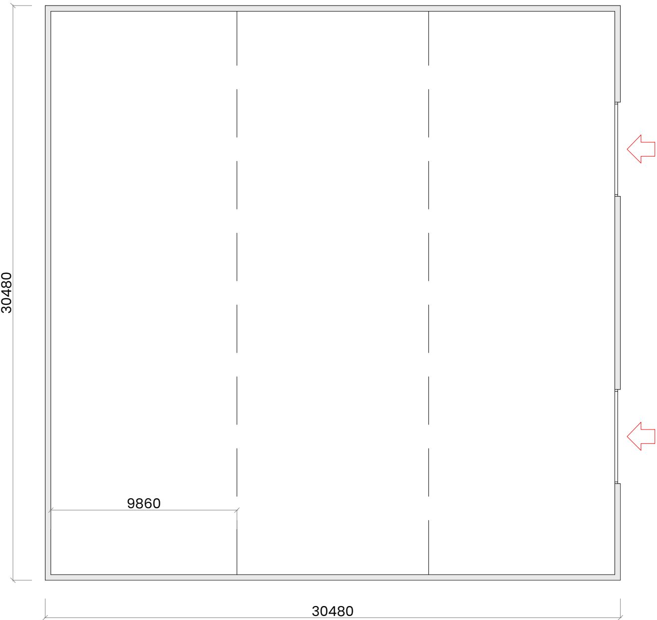
1:200 Ground Floor Plan
