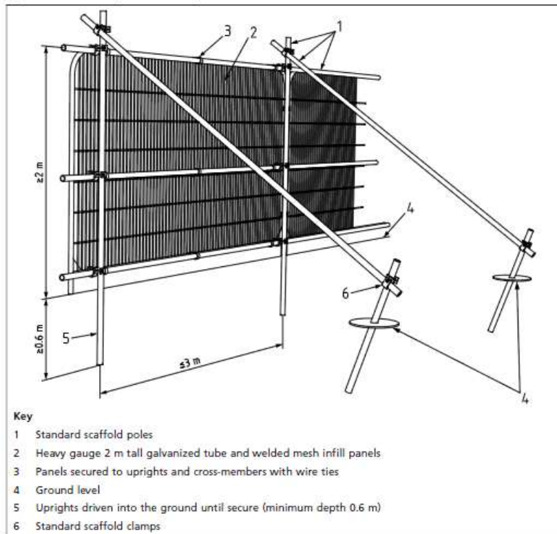
Figure 3 - Tree Protection Barrier
