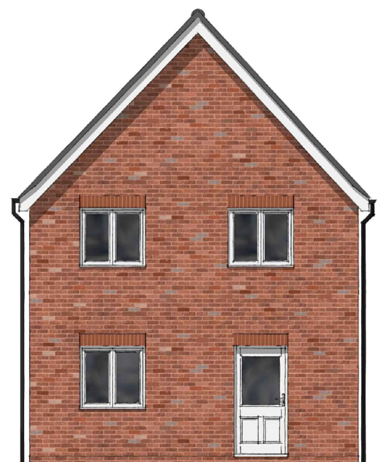
REAR ELEVATION
