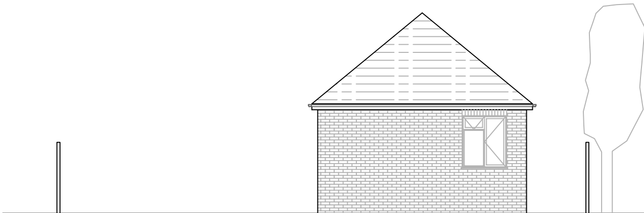
PROPOSED SIDE ELEVATION (NORTH) 1:100
