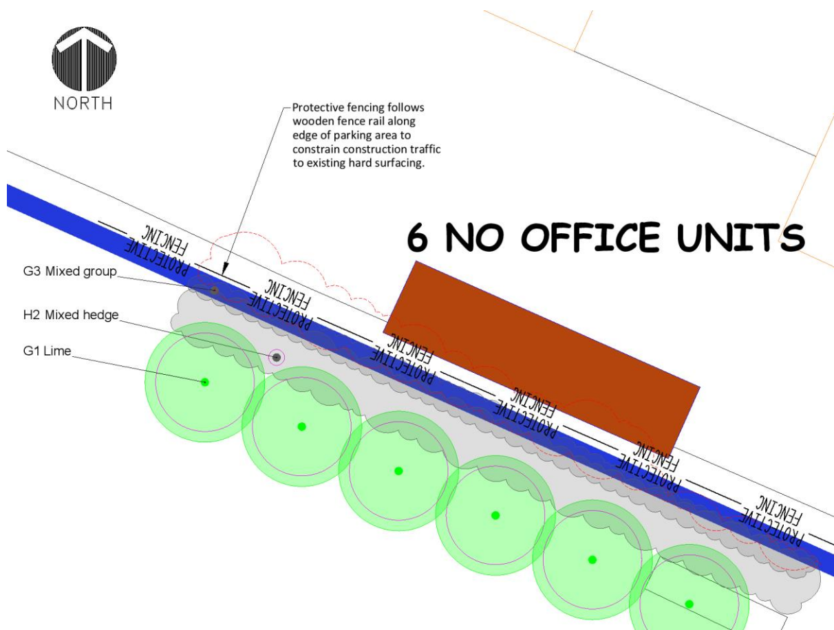
Extract from the tree protection plan showing siting of protective fencing.
