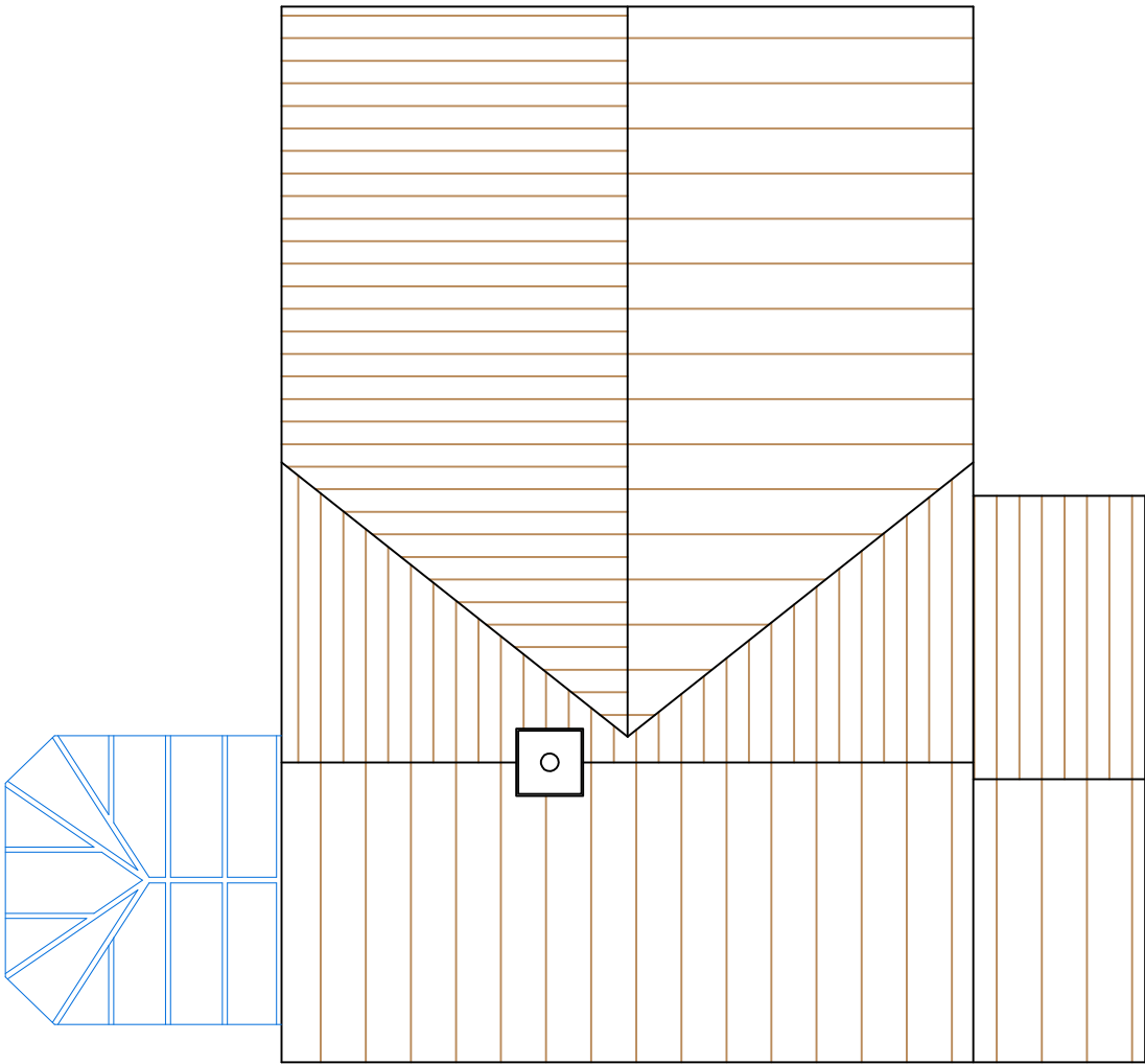
Existing Roof Plan @ 1:100 (A3)
