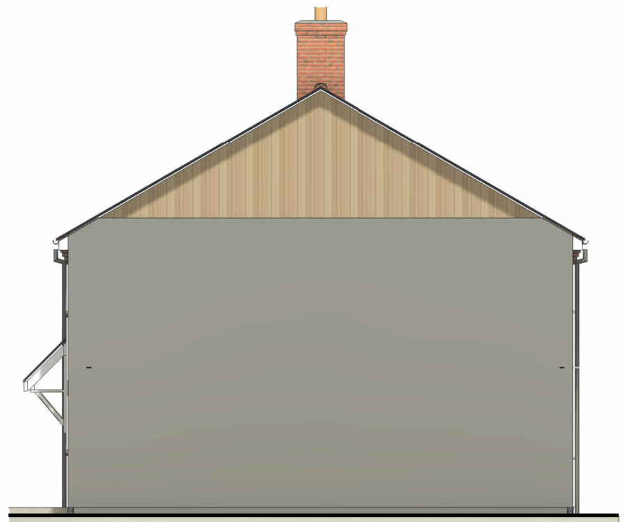
Side 1 Elevation
