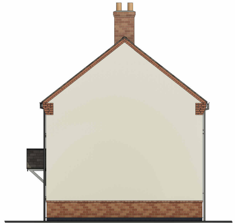
Side 2 Elevation
