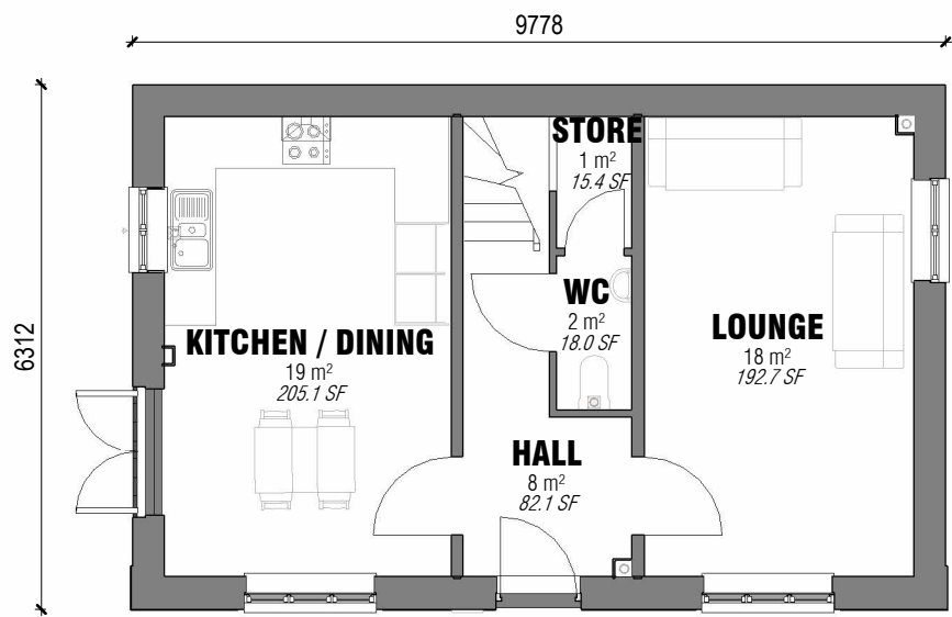
Ground Floor Plan Copy 1
