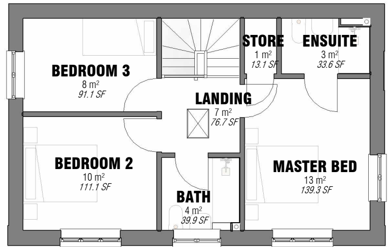
First Floor Plan Copy 1
