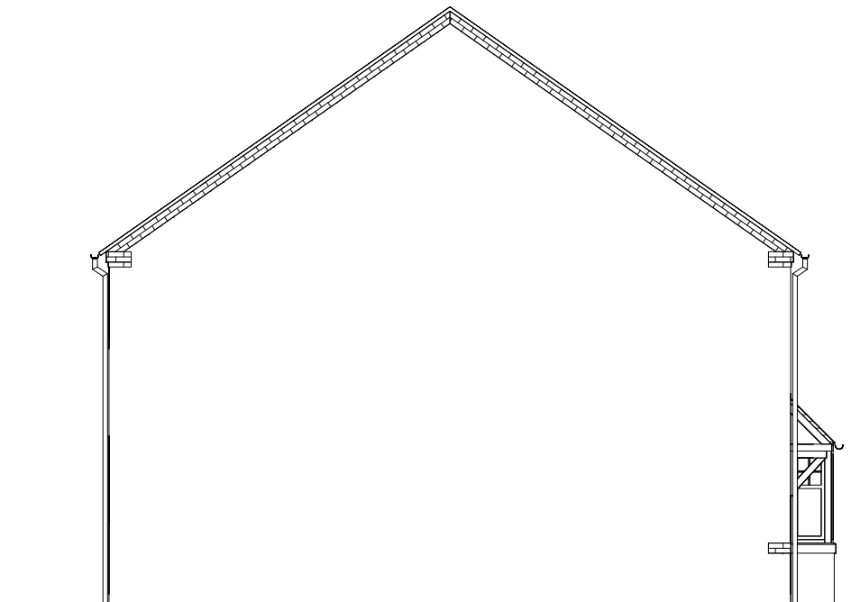
Left Elevation
