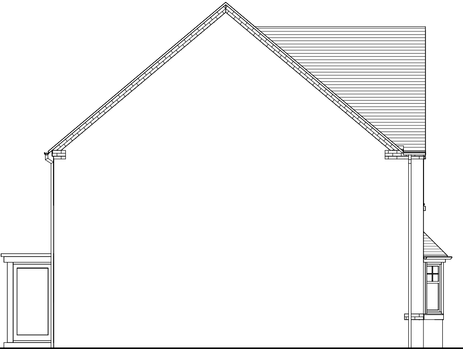
Left Elevation
