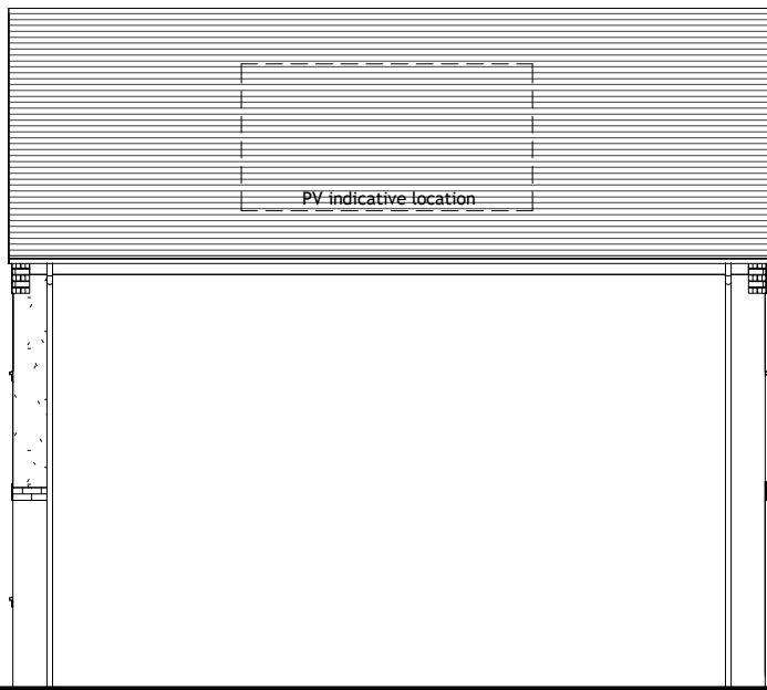
Rear Elevation
