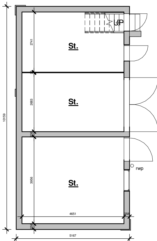
Existing GF Plan - 1:100
