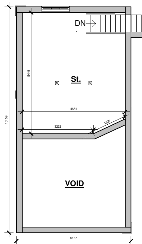
Existing FF Plan - 1:100
