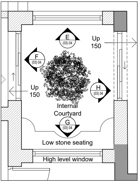
Key Plan Scale 1:50
