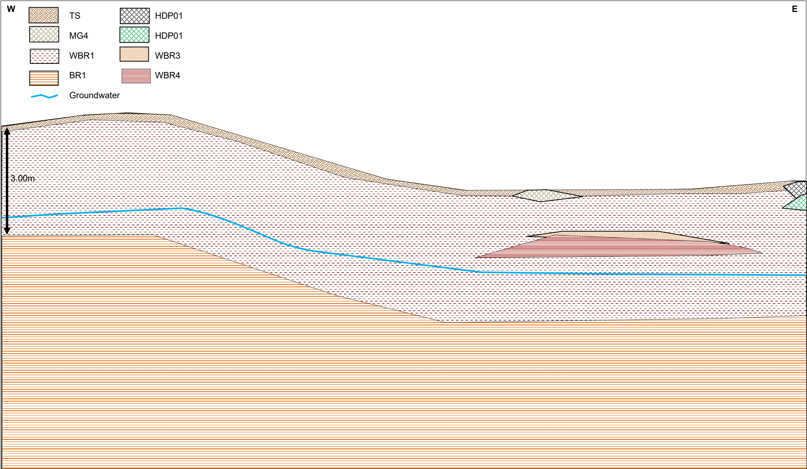
Figure 7.1 Schematic Drawing of Ground Conditions
