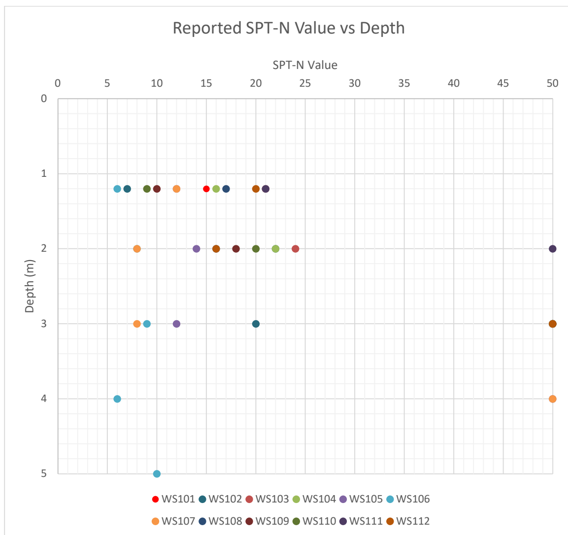
Figure 8.3 SPT N value vs reduced depth
