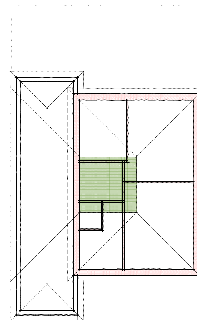
PROPOSED ROOF LAYOUT
