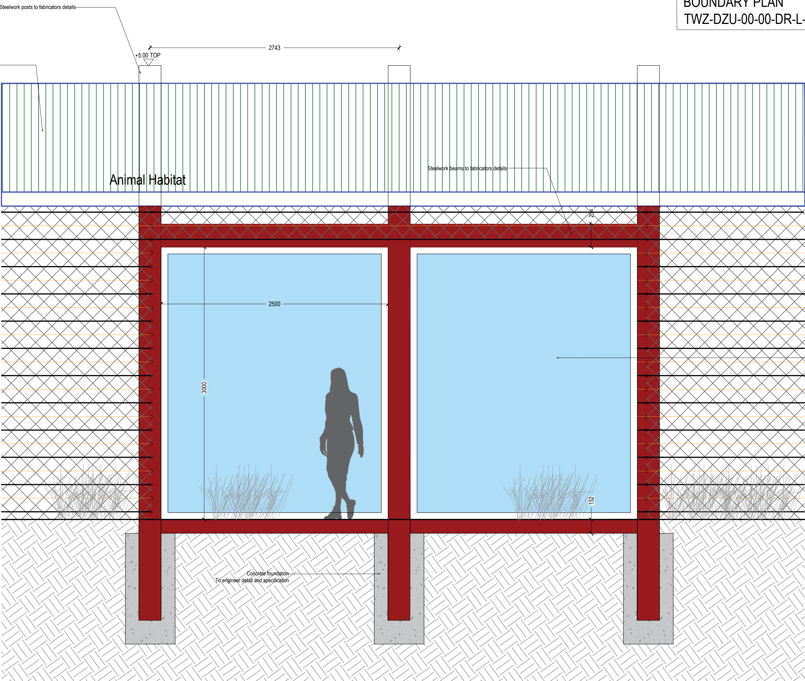
F3 3m high Viewing window intergrated into containment - Elevation
