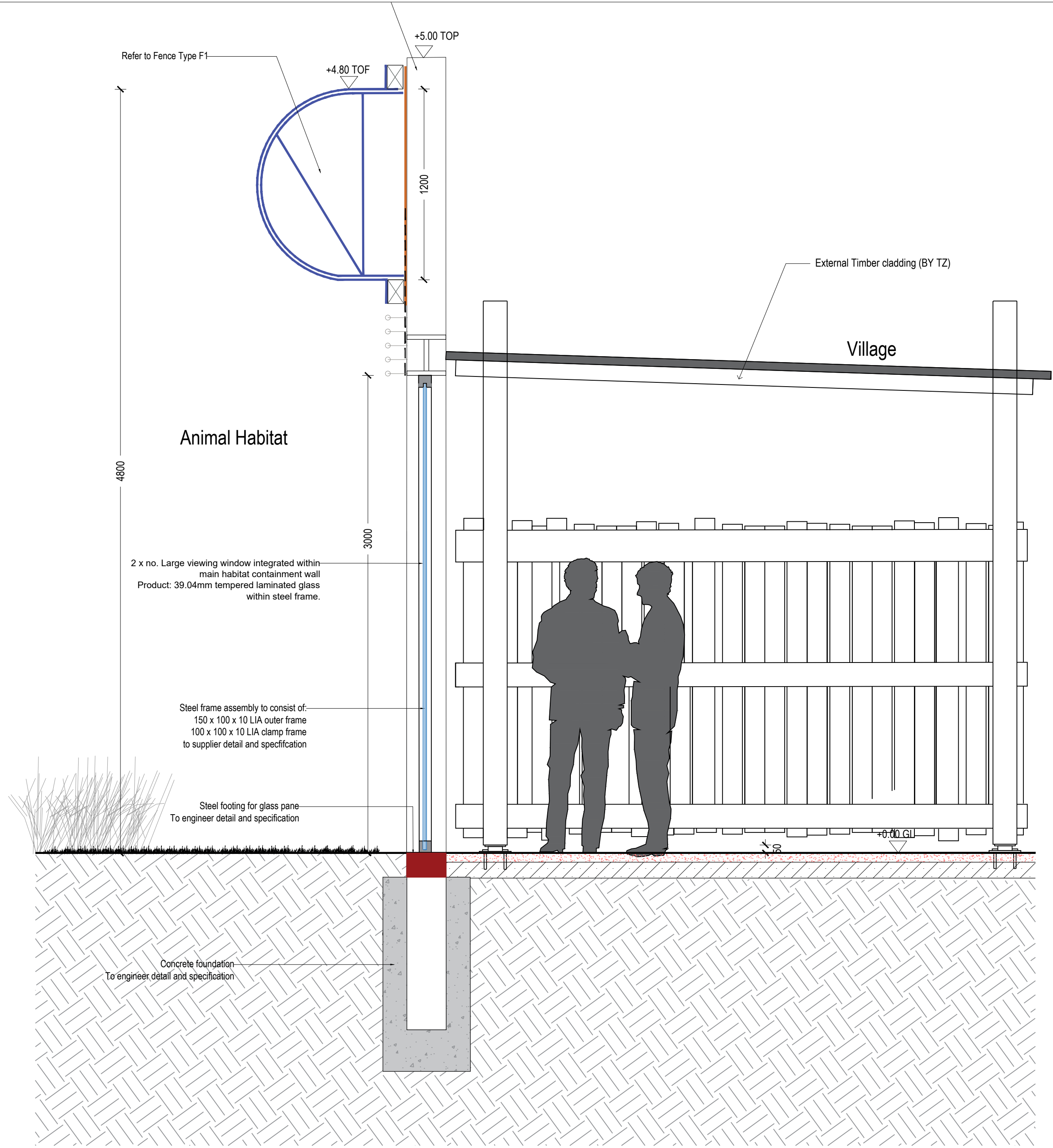
F3 3m high Viewing window intergrated into containment - Section
