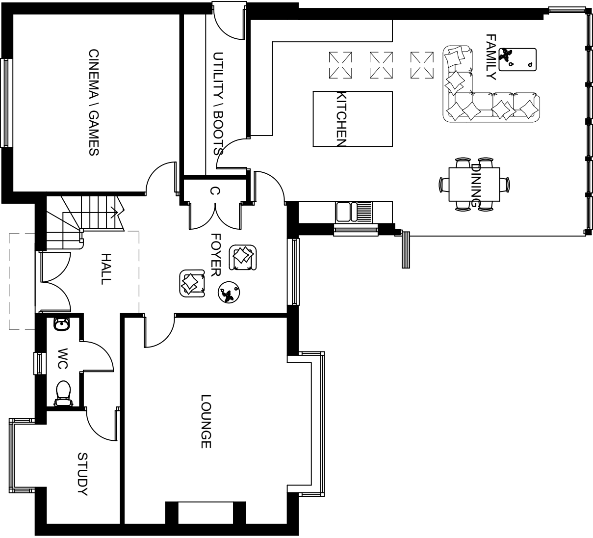
GROUND : UNIT 1 TOTAL 2585 sq ft
