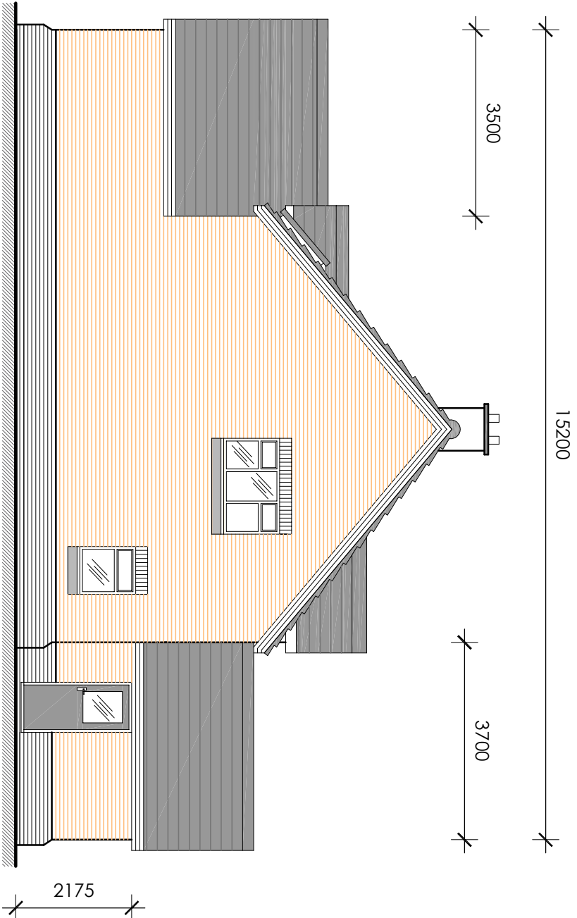
Side Elevation
