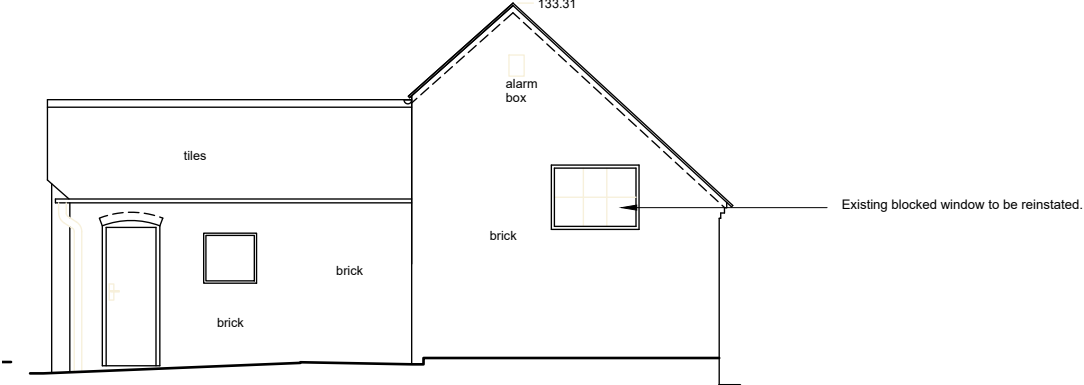
South elevation
