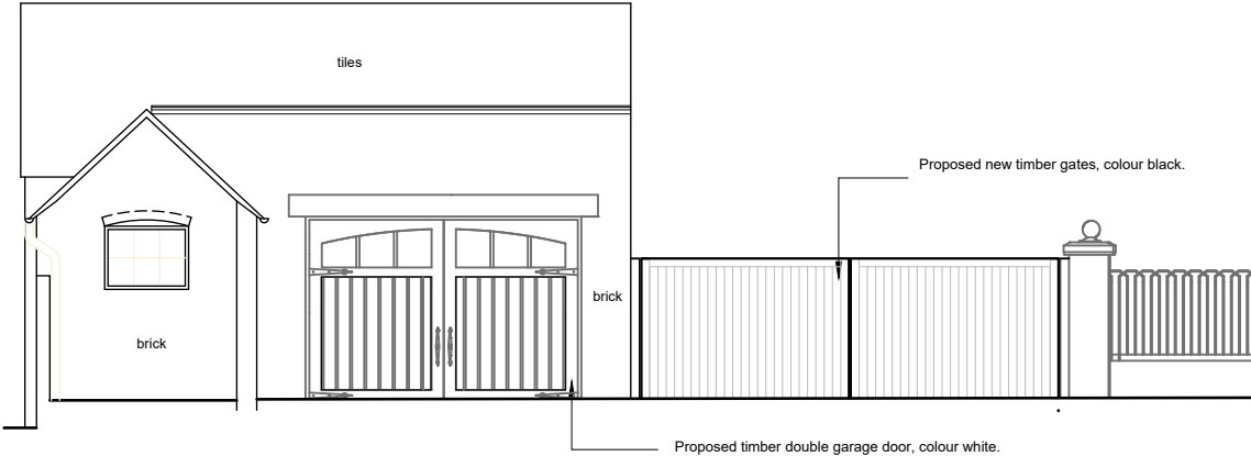
West elevation
