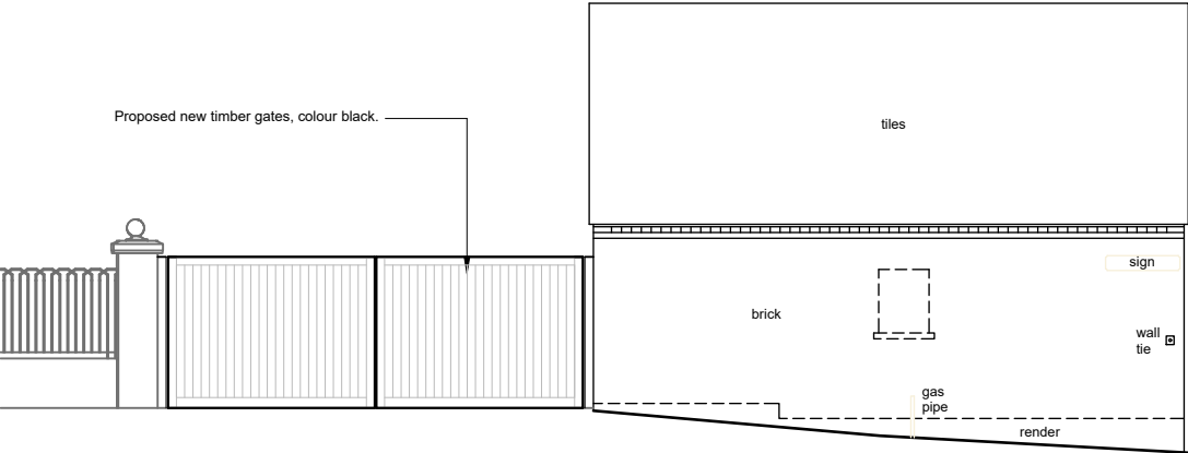
East elevation
