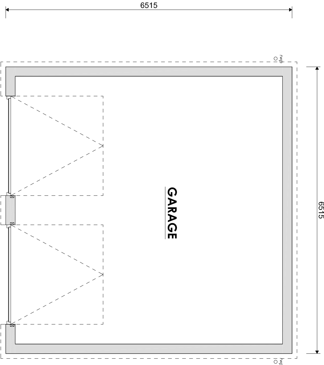
FLOOR PLAN
