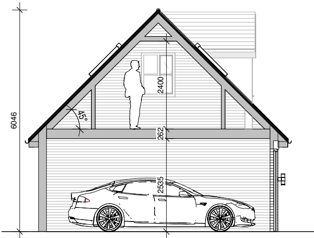
Section
