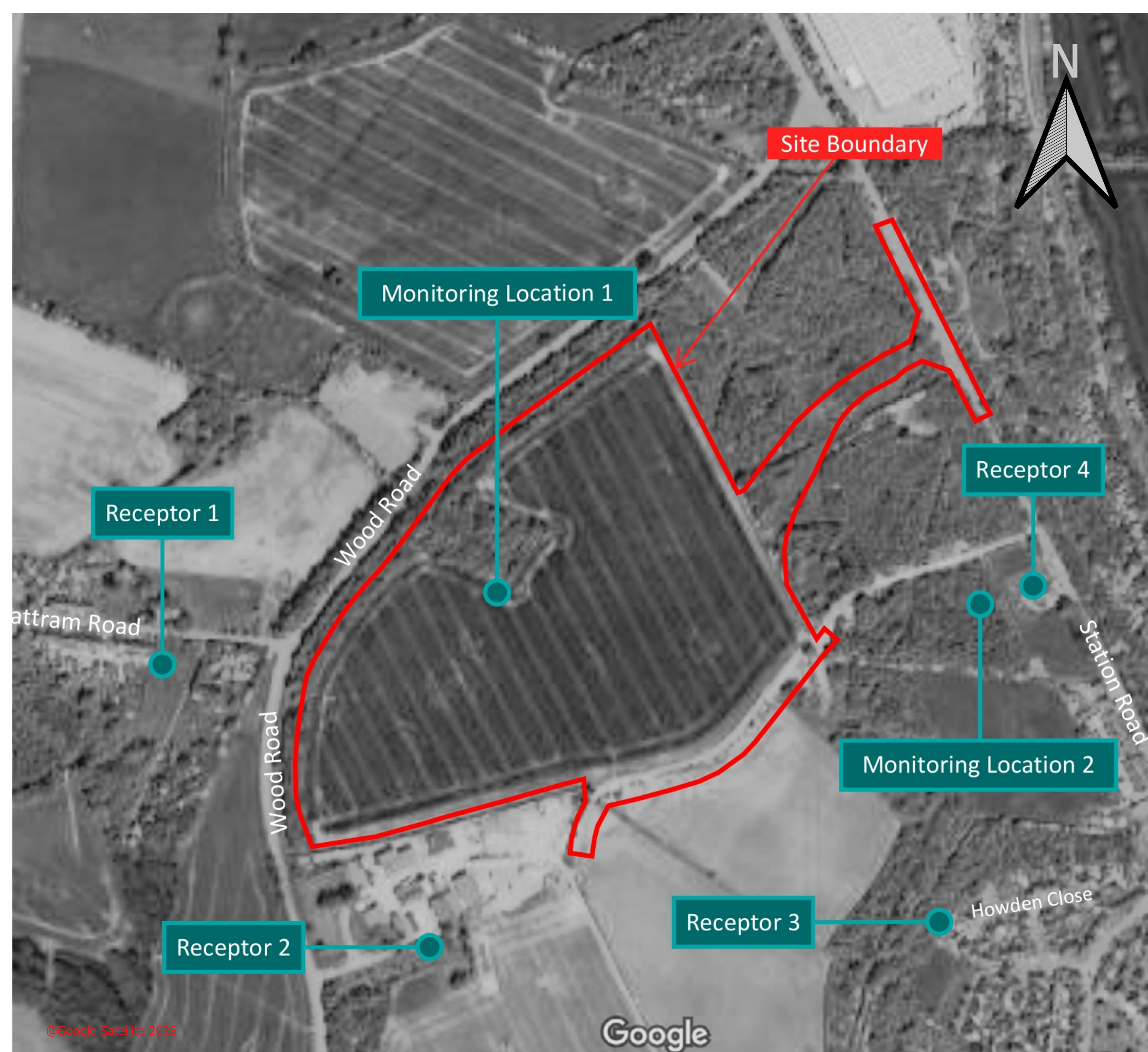
Figure 9.1 - Receptor & Noise Monitoring Locations
