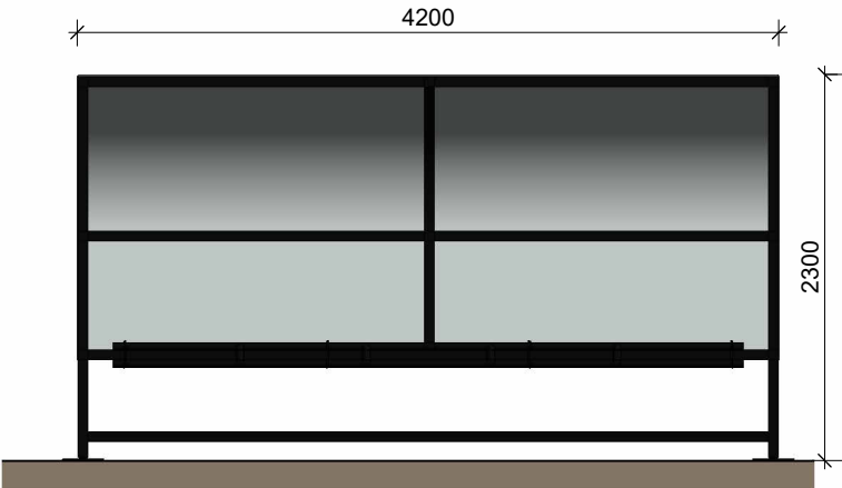
Typical Smoking Shelter - Front 1 : 50
