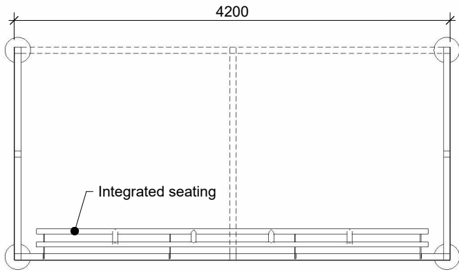
Typical Smoking Shelter - Plan 1 : 50
