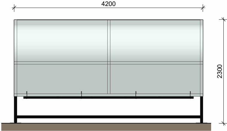
Typical Smoking Shelter - Rear 1 : 50
