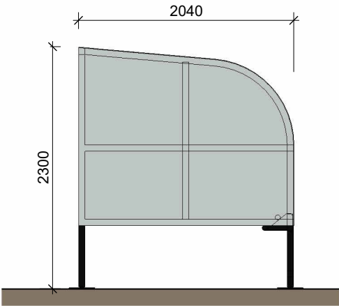
Typical Smoking Shelter - Side 2 1 : 50
