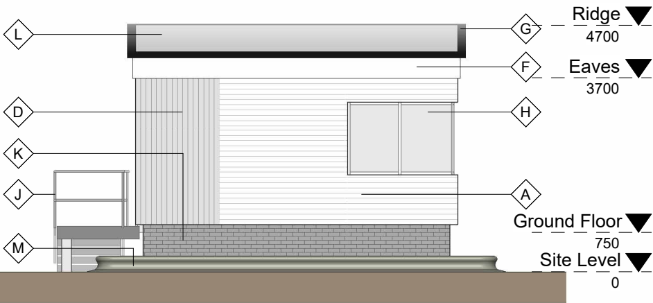
North-East Elevation
