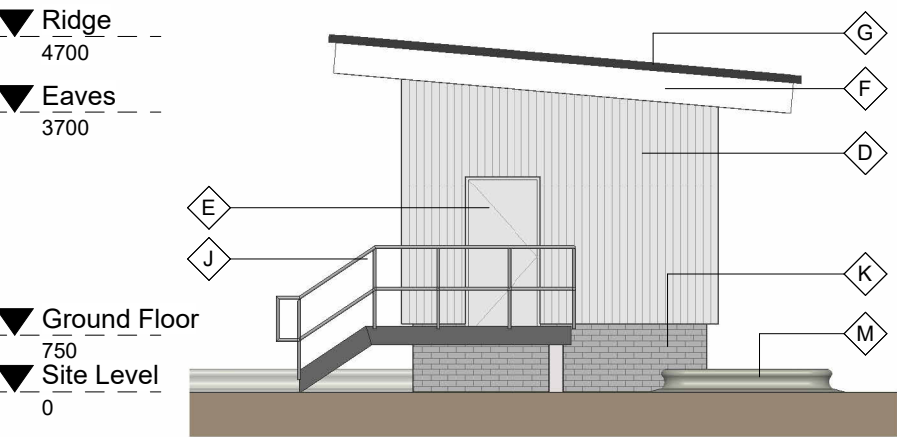
South-East Elevation
