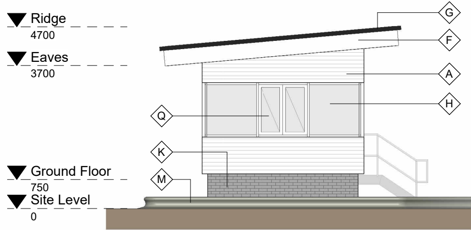
NorthWest Elevation
