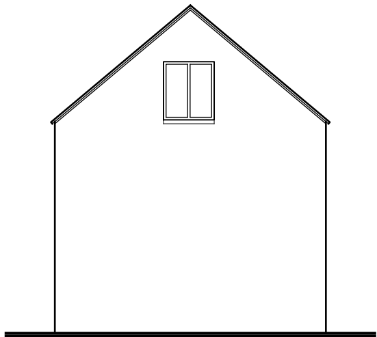
SIDE ELEVATION
