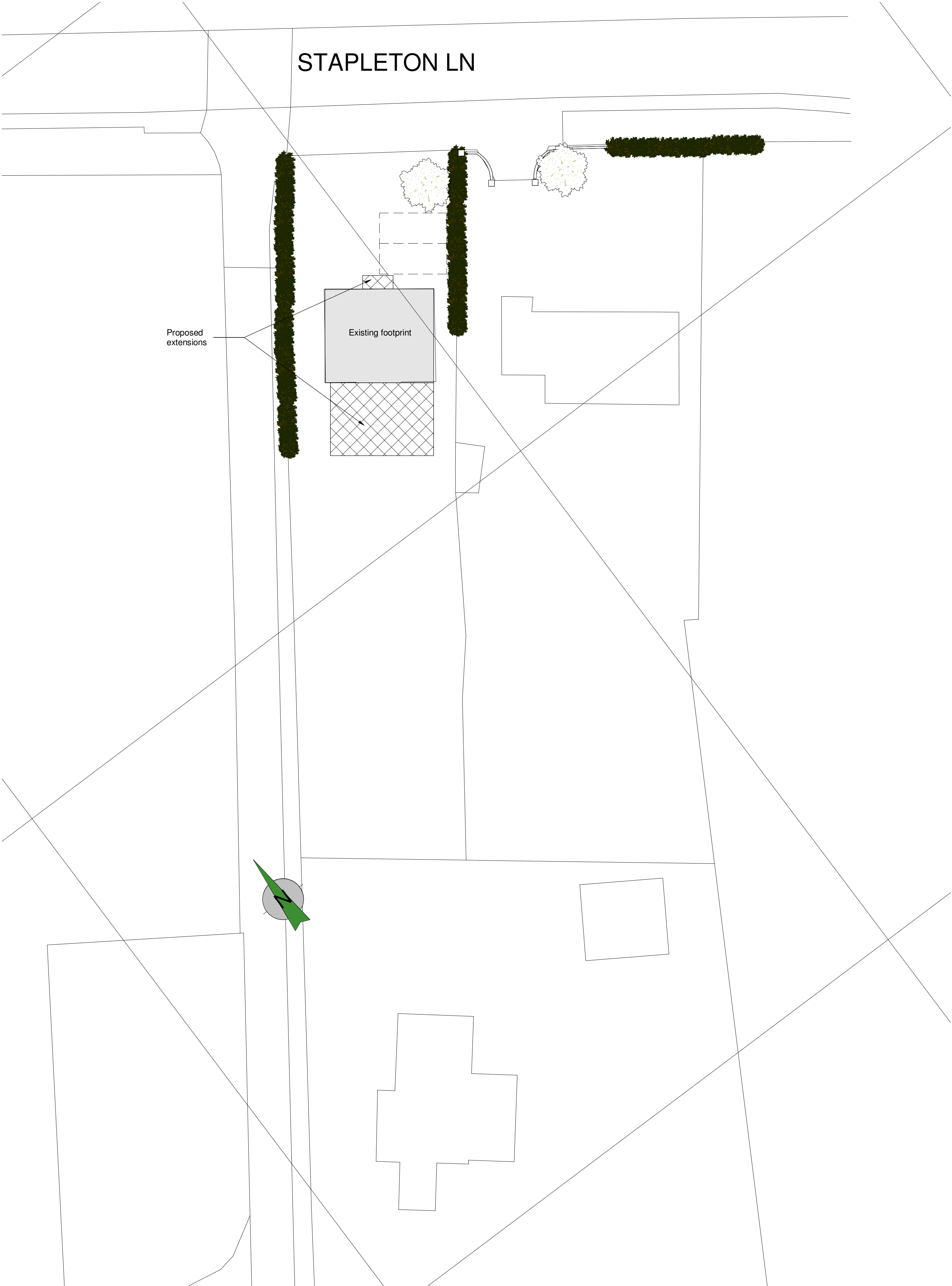
BLOCK PLAN - 1:200
