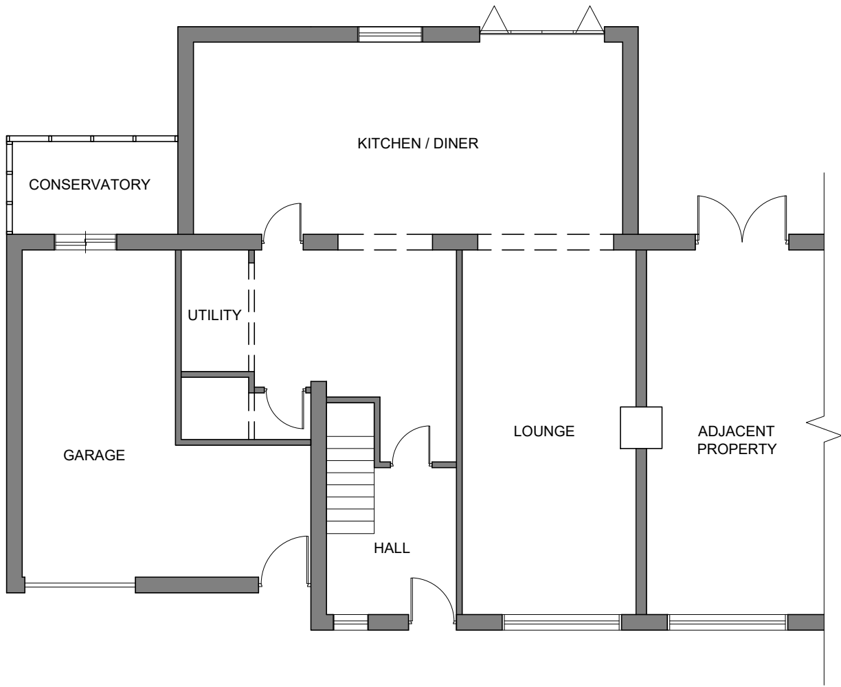
B 01 GROUND FLOOR PLAN (Proposed)
