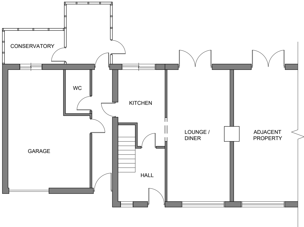
B 03 GROUND FLOOR PLAN (Existing)
