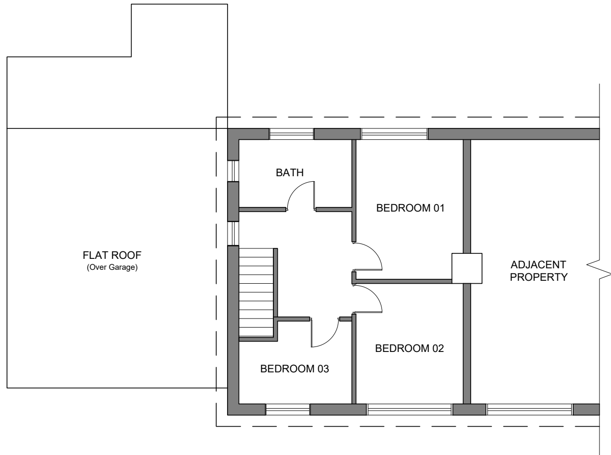
B 04 FIRST FLOOR PLAN (Existing)
