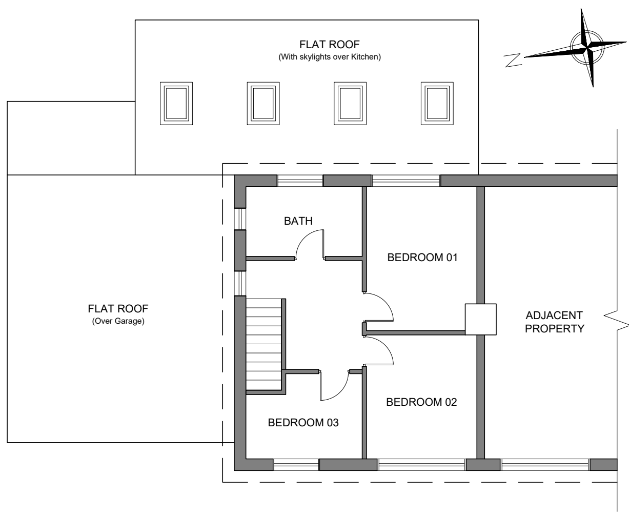
B 02 FIRST FLOOR PLAN (Proposed)
