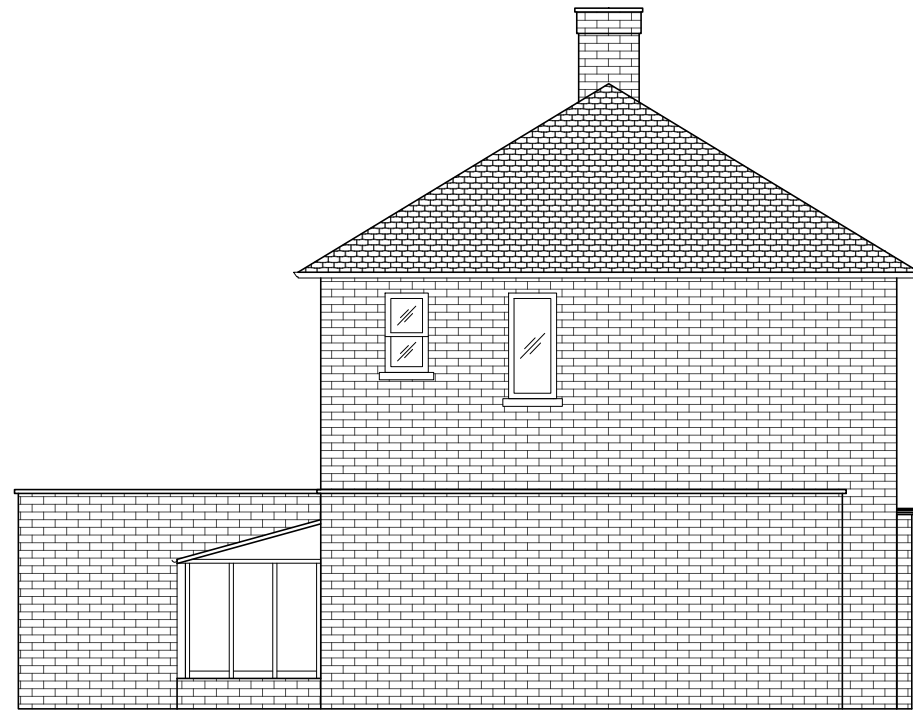
D 03 NORTH ELEVATION (Proposed)
