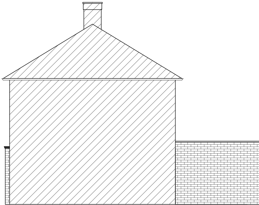
D 04 SOUTH ELEVATION (Proposed)
