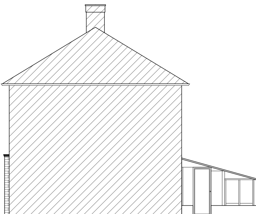
C 04 SOUTH ELEVATION (Existing)
