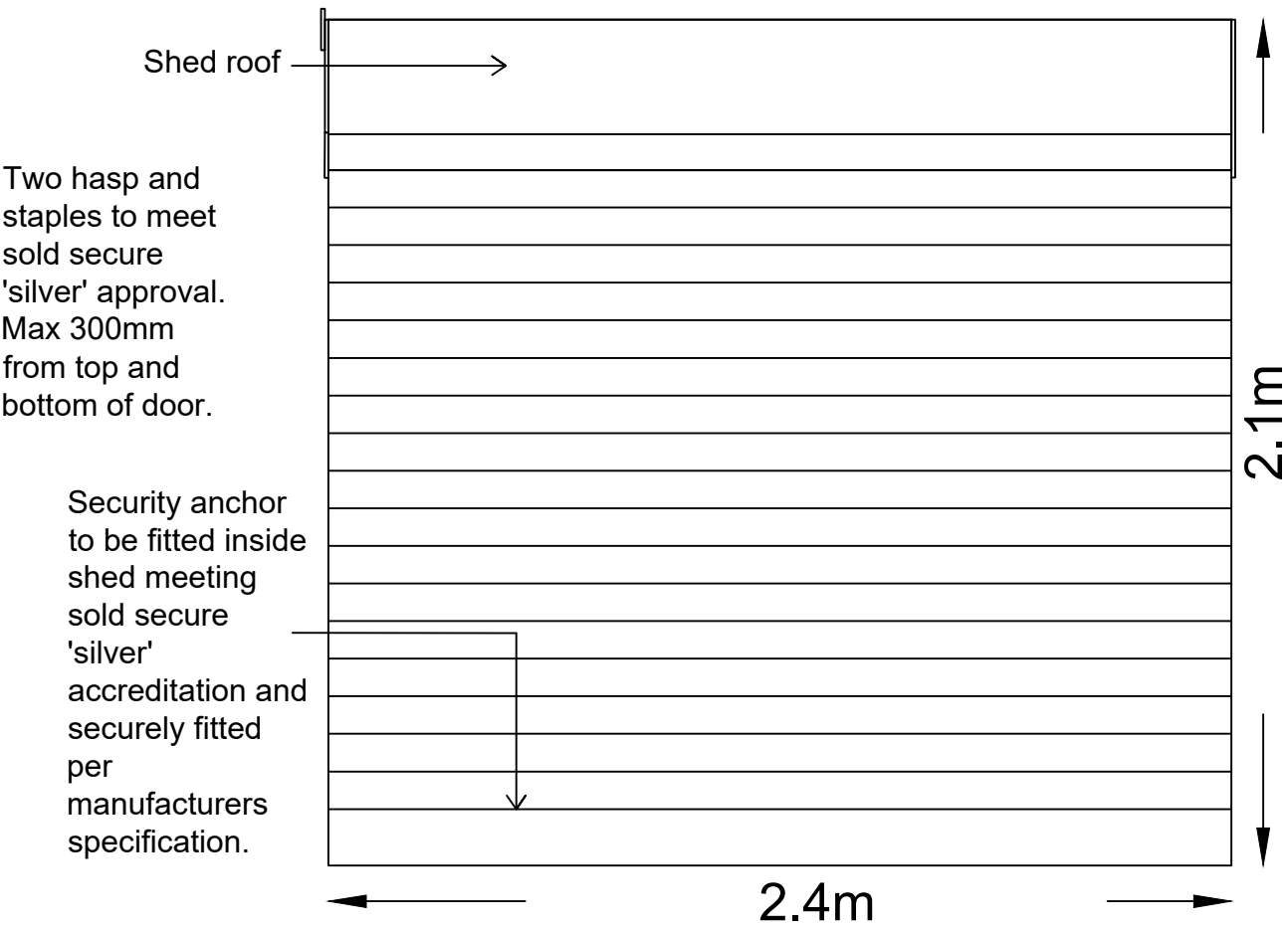
Side Elevation
