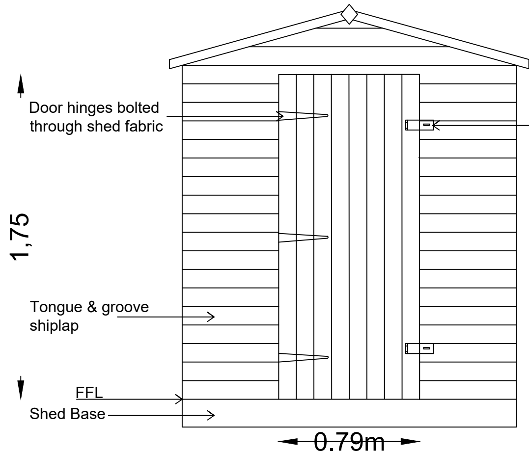
Rear Elevation
