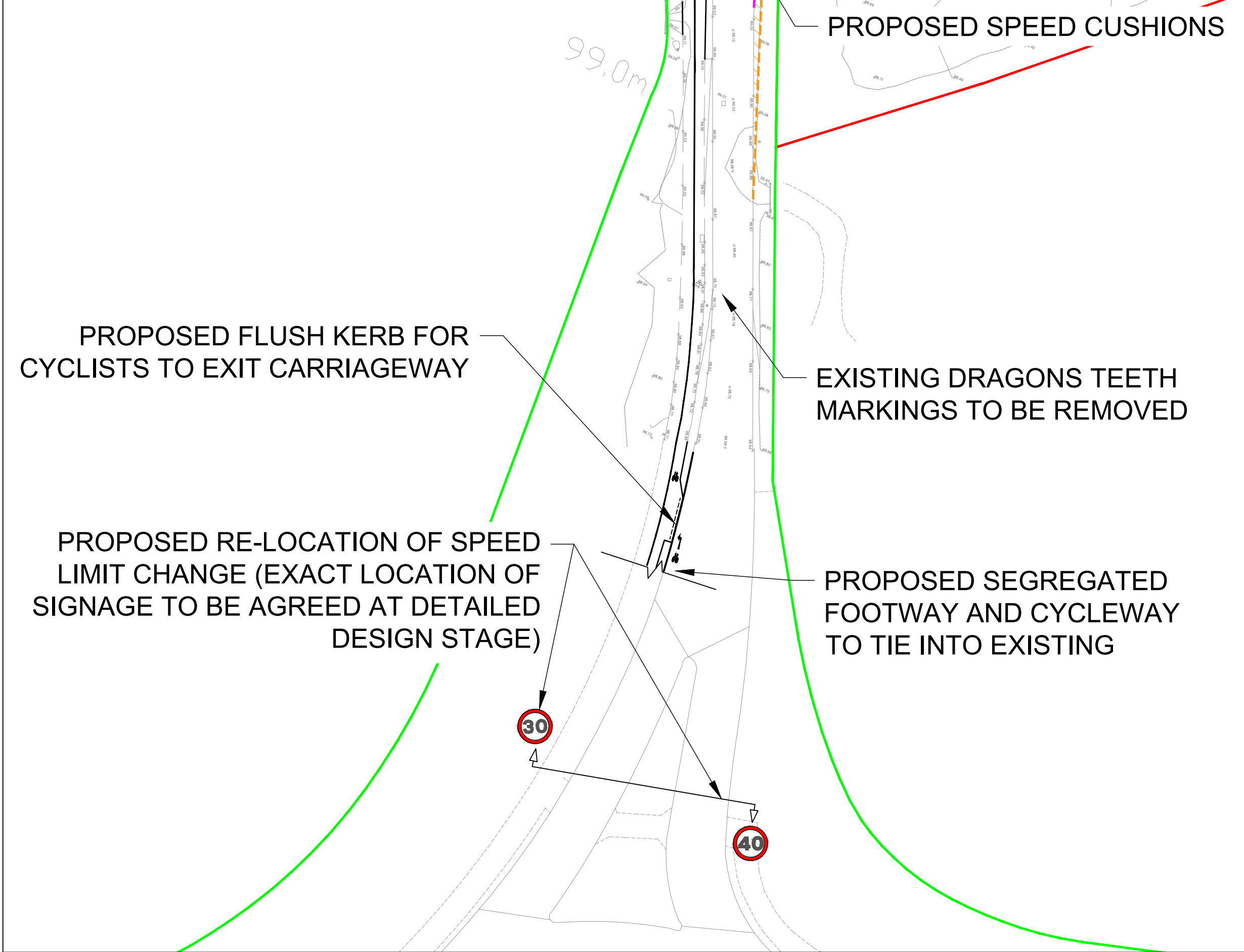
THE COMMON, BARWELL SITE ACCESS PLAN 1:500
