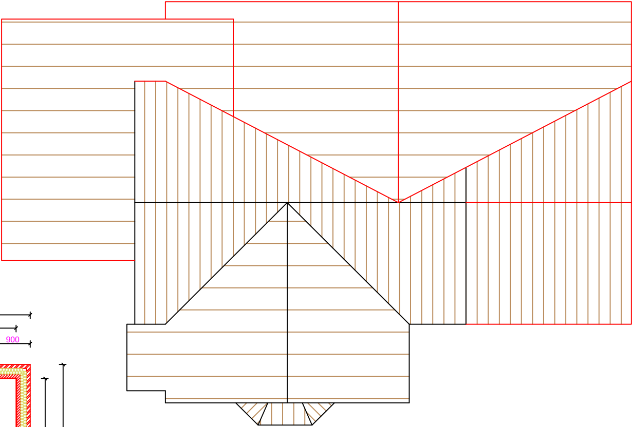
Proposed Roof Plan @ 1:100 (A3)
