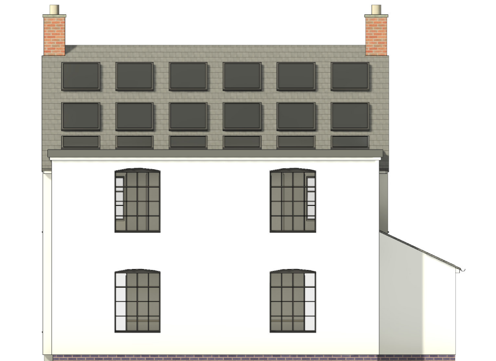
Rear Elevation
