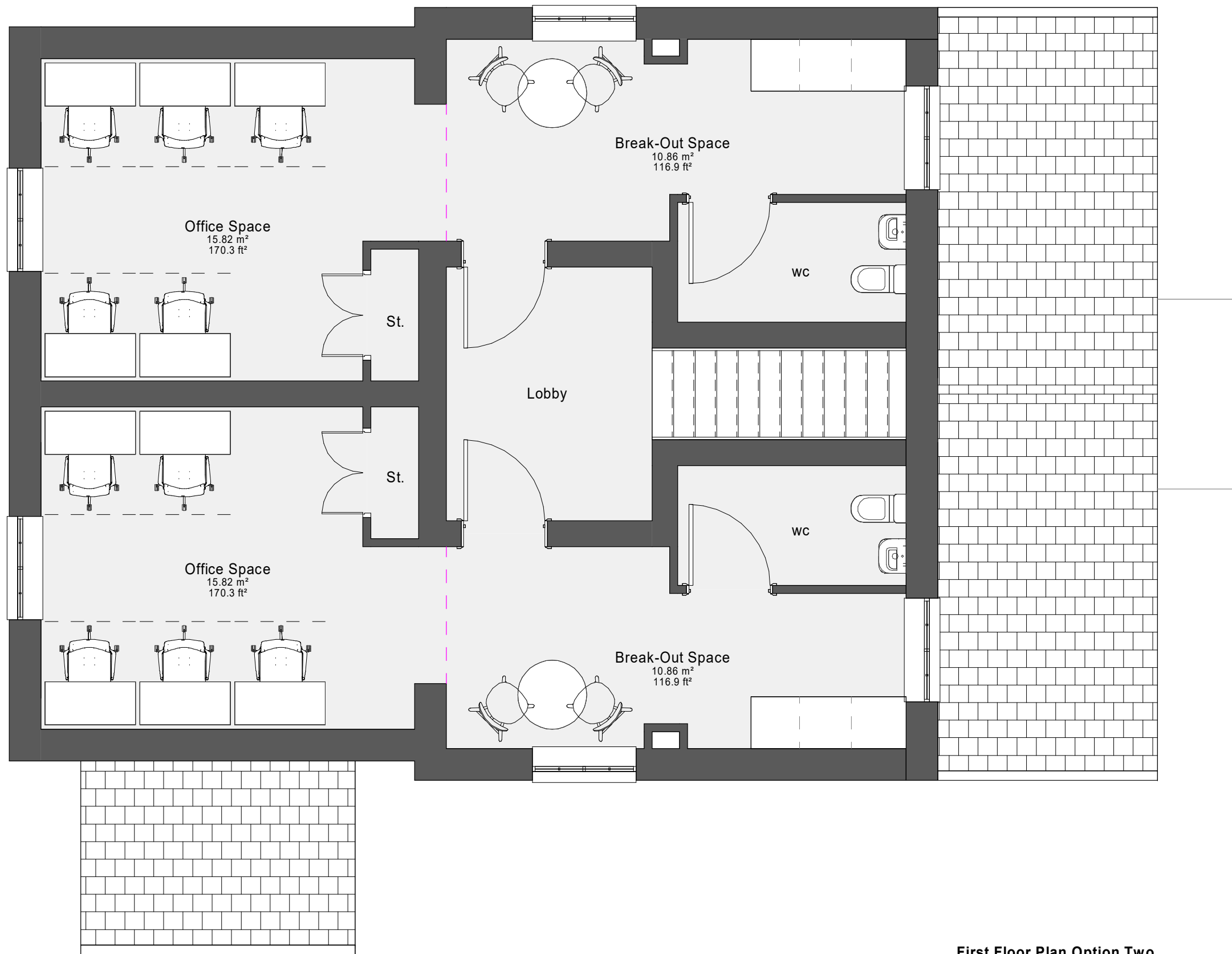
First Floor Plan Option Two Each Unit = 32m 2
