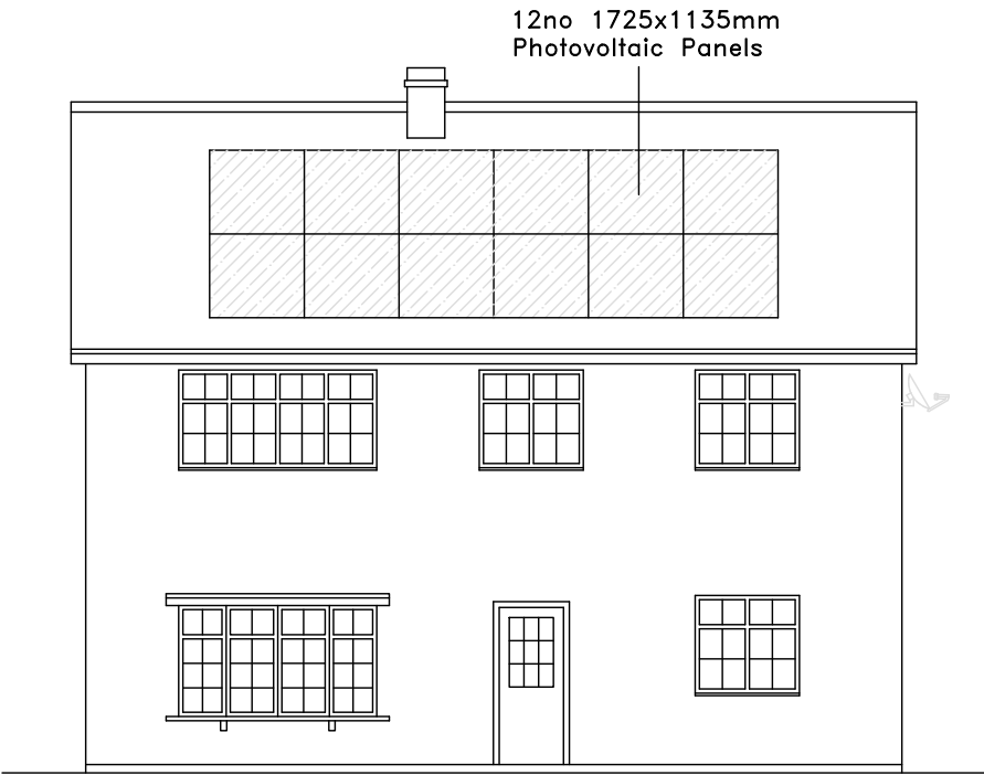
Front (South) Elevation
