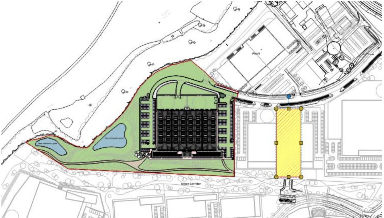
Figure 2 – location of existing haul road and site compound marked in yellow.
