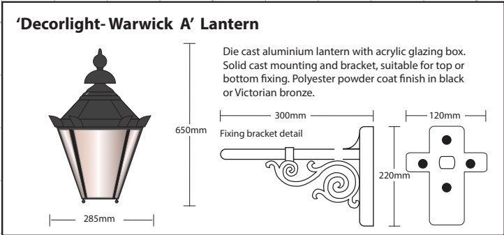
G ONE X NEW LANTERN TO ENTRANCE. SIZE. 0.28m x 650mm. H.A.G. 2.9m.
