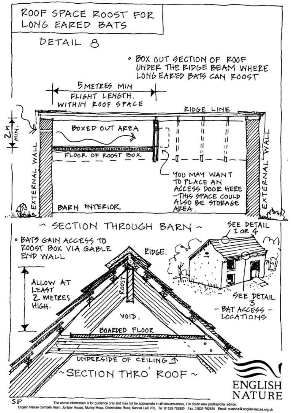
ROOF SPACE ROOST FOR LONG EARED BATS.
