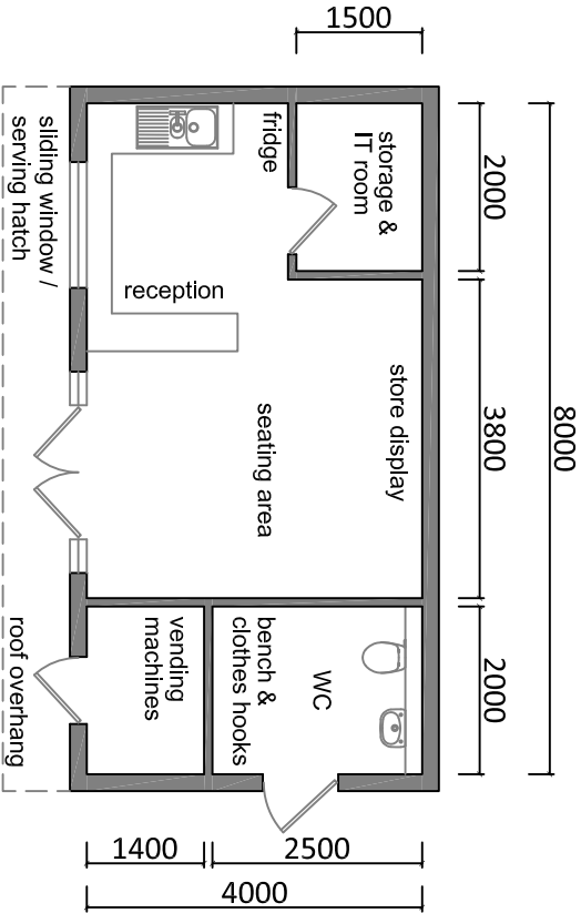
Floor Plan
