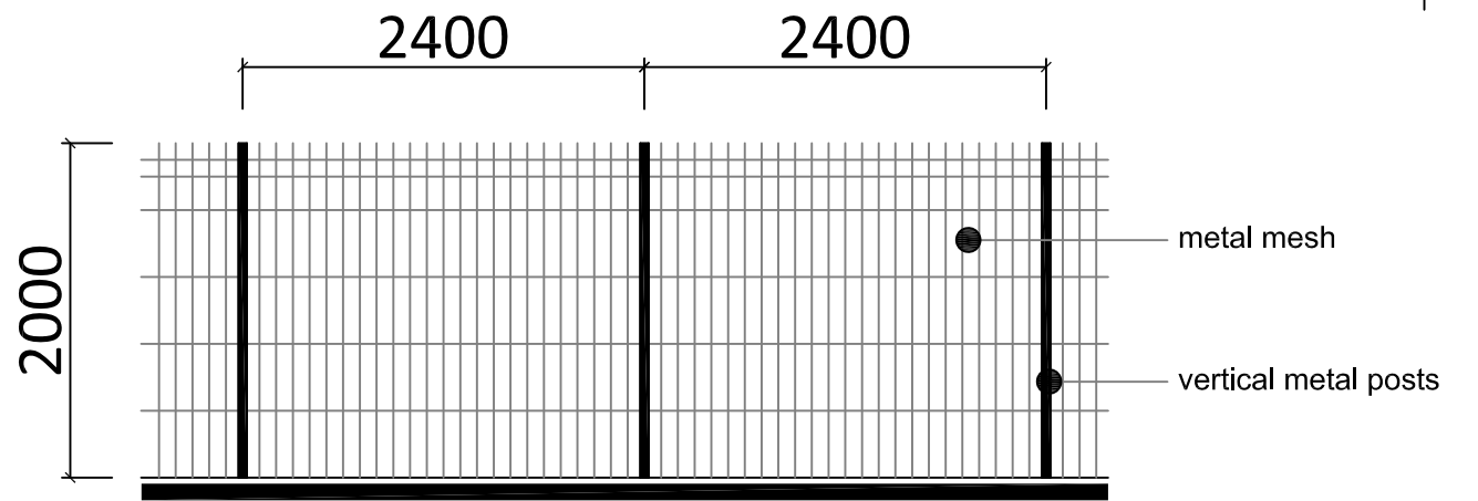
Front Elevation 1:50
