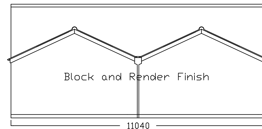
Proposed Left Elevation
