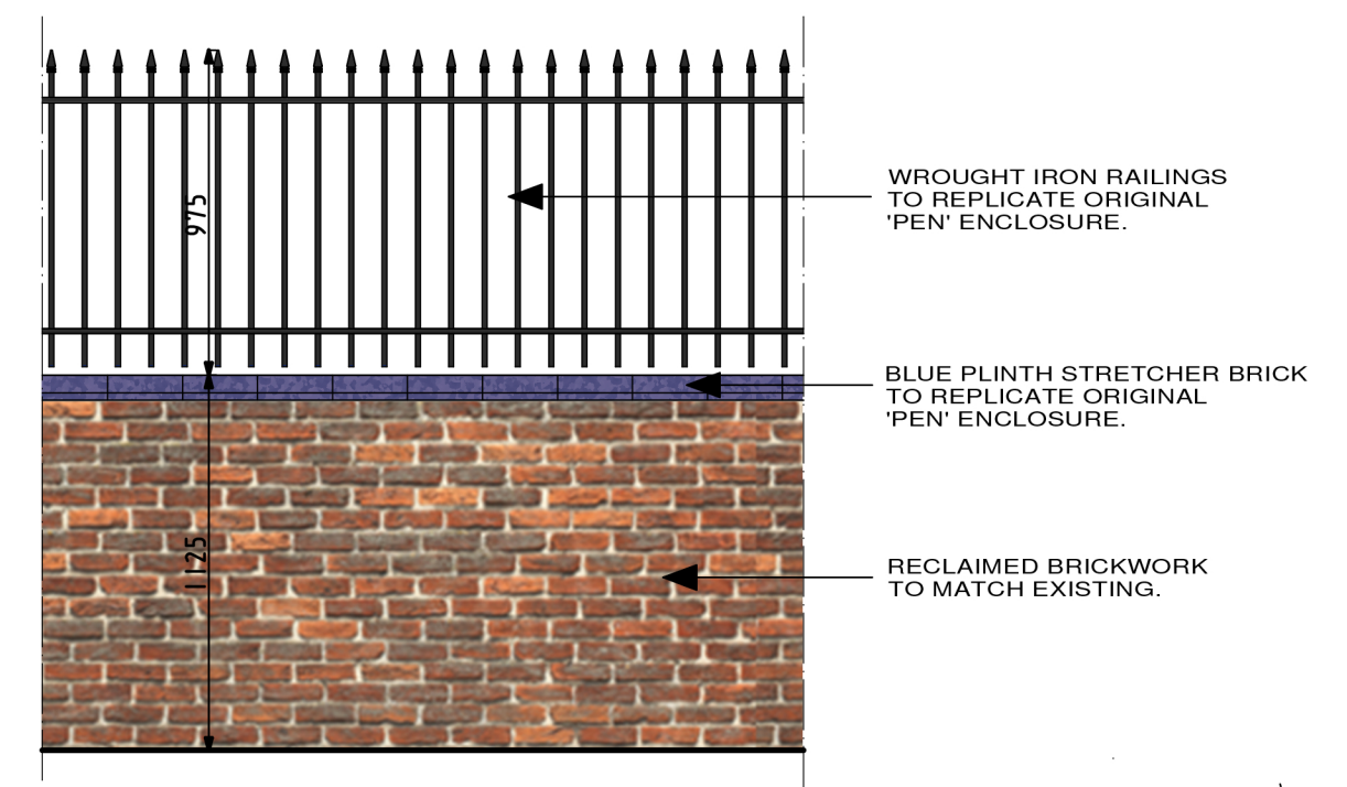
1.125m BRICKWORK WITH 0.975m WROUGHT IRON RAILINGS.
