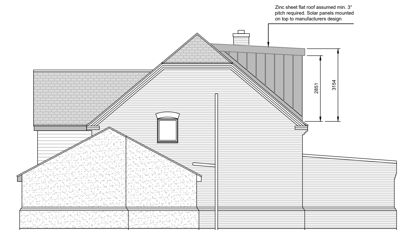
Proposed Right Elevation
