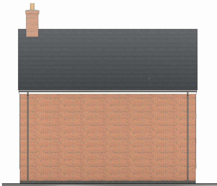
Rear Elevation
