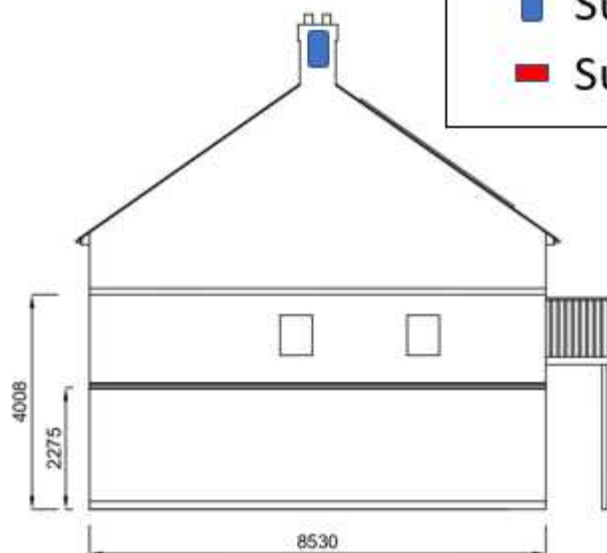
Proposed Right Elevation (South East)
