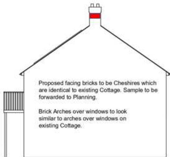
Proposed Left Elevation (North West)
