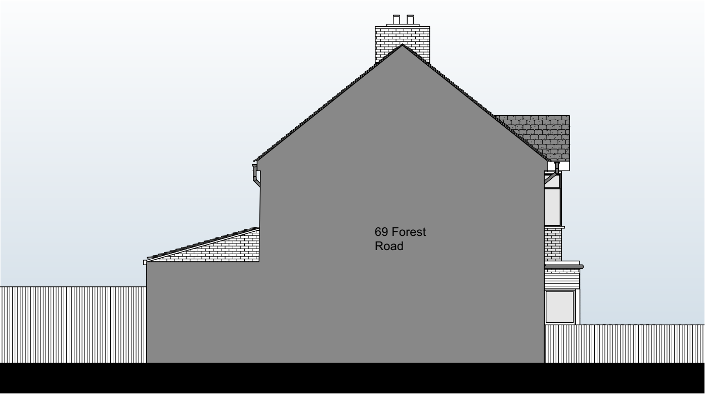
Existing South - West Elevation
