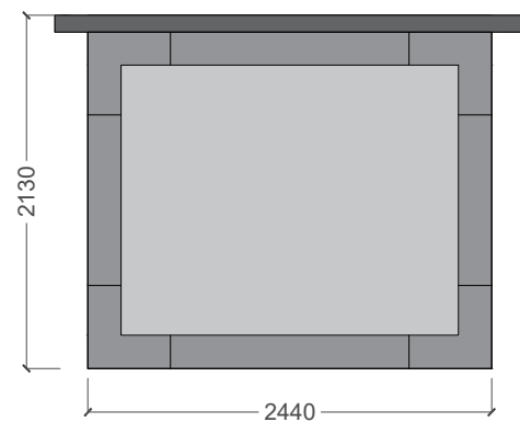
East Elevation
