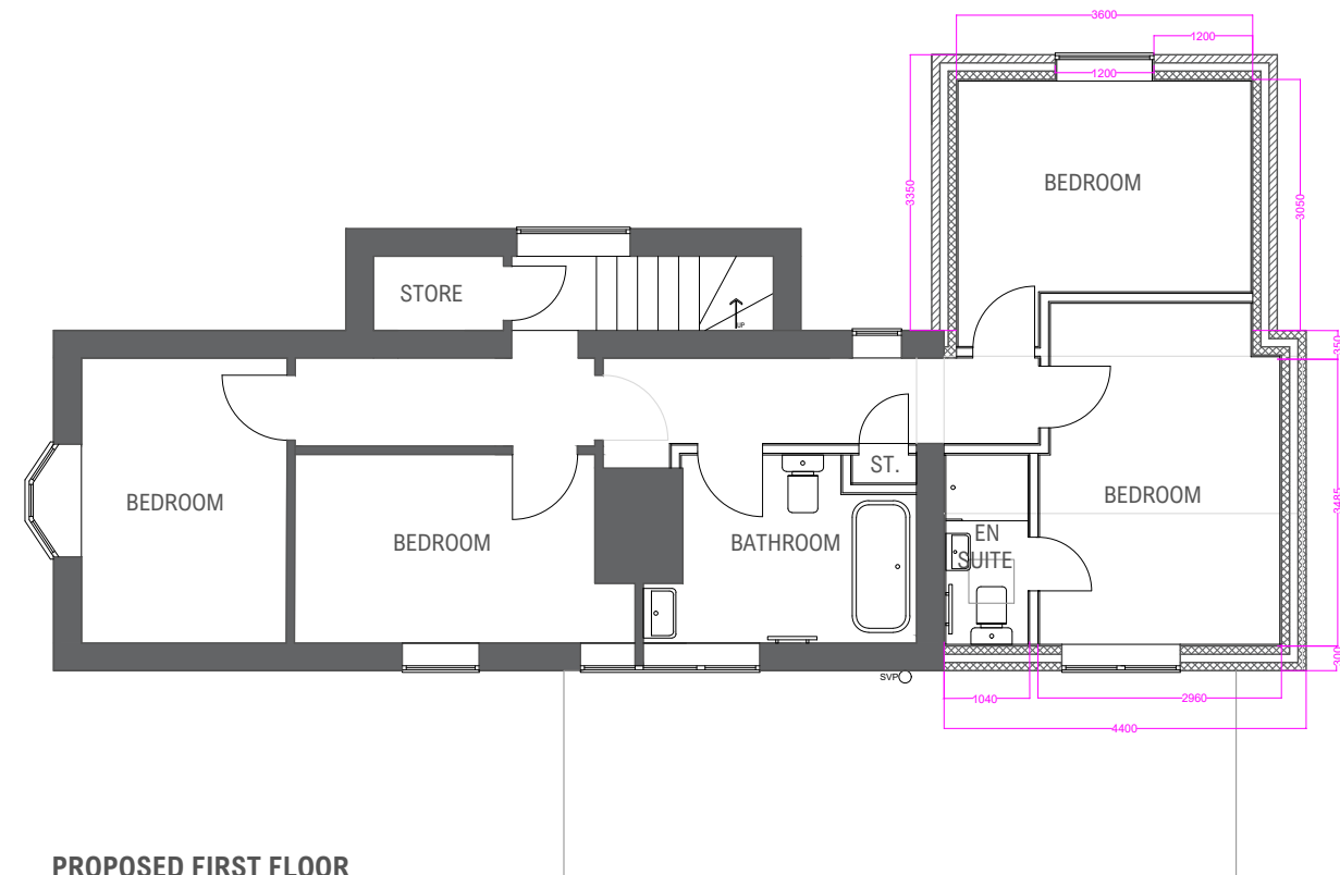
PROPOSED FIRST FLOOR
