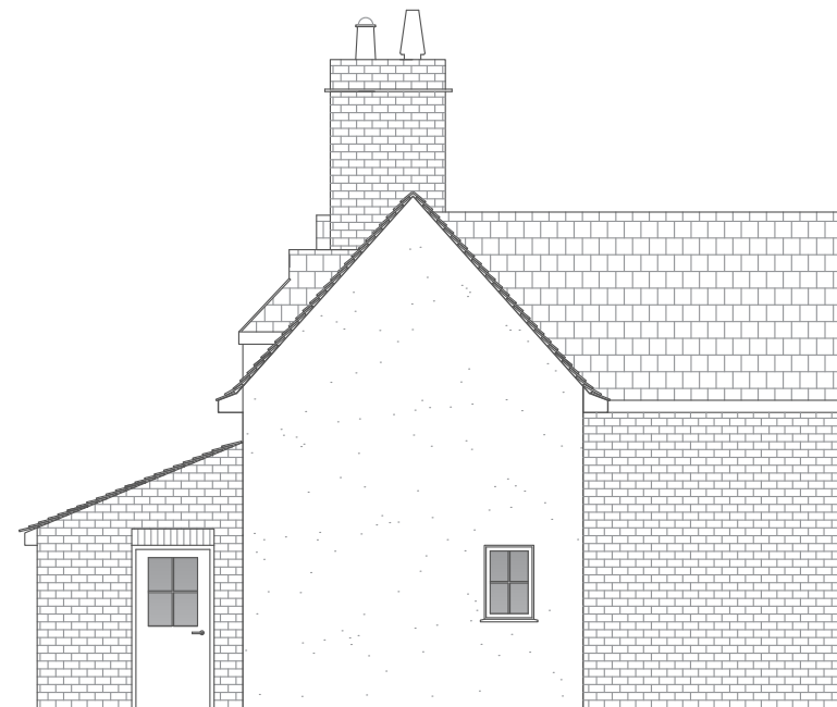
PROPOSED NORTHERN ELEVATION
